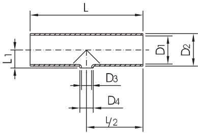
Redukovani T-komad reducing tee SSS
